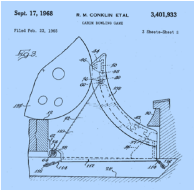
Among Ted Rebain’s personal effects was this diagram that best displays the bumper apparatus used for the Carom Bowling Game. The entire 9 page report is available at freepatentsonline.com . Provided by Dave Williams
